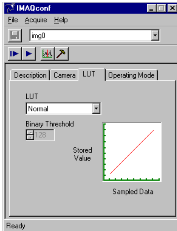
Figure 5-5. LUT Tab Settings
