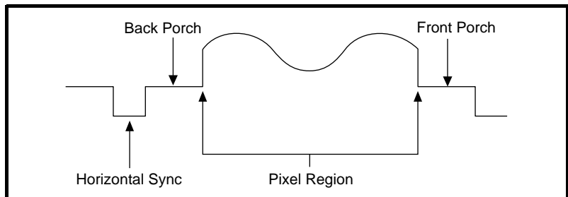
Figure 3-2. Video Line
