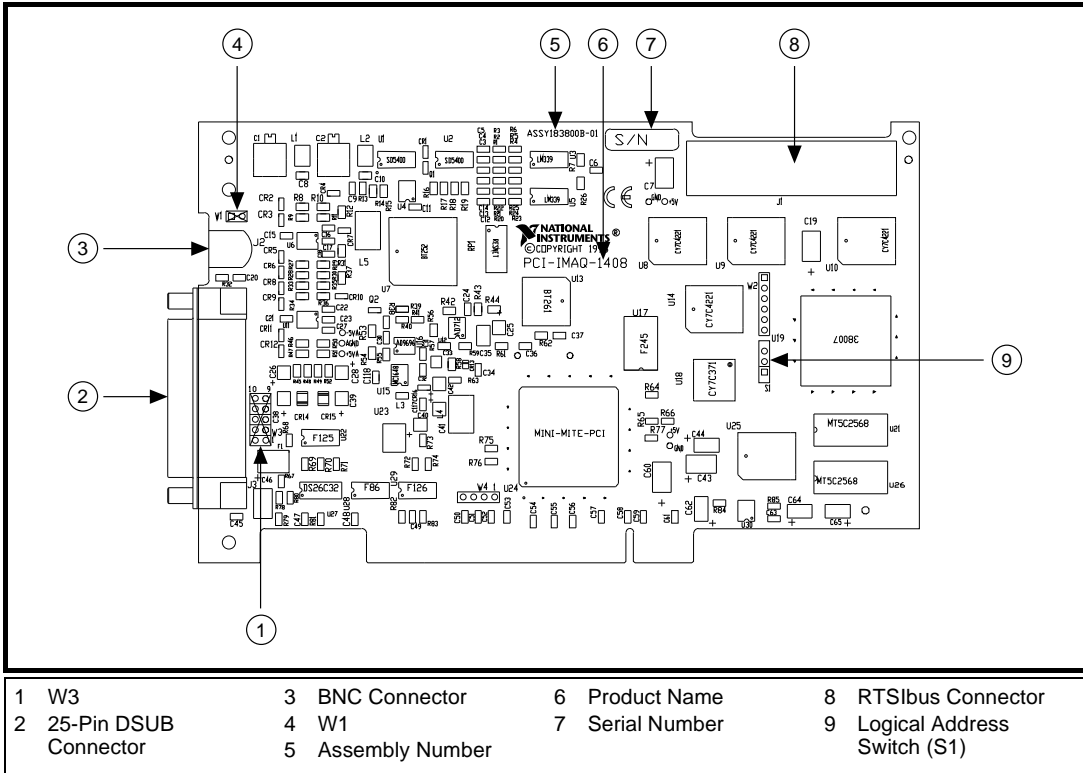
Figure 2-1. Parts Locator Diagram
