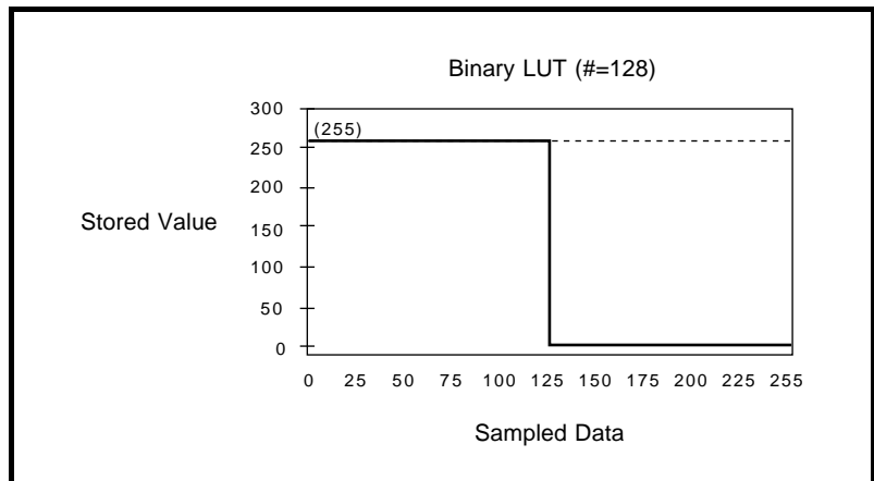
Figure 5-11. Inverse Binary LUT
