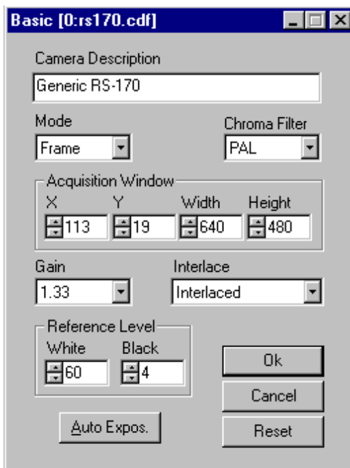
Figure 5-3. Basic Camera Settings
